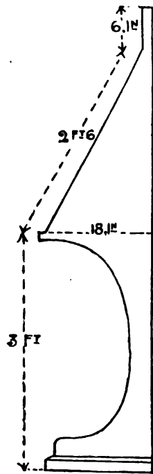
FIG. 32.—Wall Newspaper Stand, showing Dimensions (Section 164).
